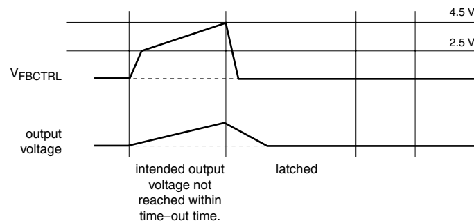
Fig 14. Time-out protection (signals), latched in the TEA1751AL
