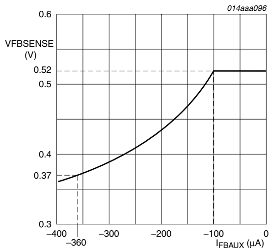
Fig 17. Overpower protection curve
