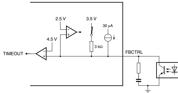
Fig 12. Time-out protection circuit
