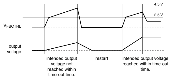
Fig 13. Time-out protection (signals), safe restart in the TEA1751A
