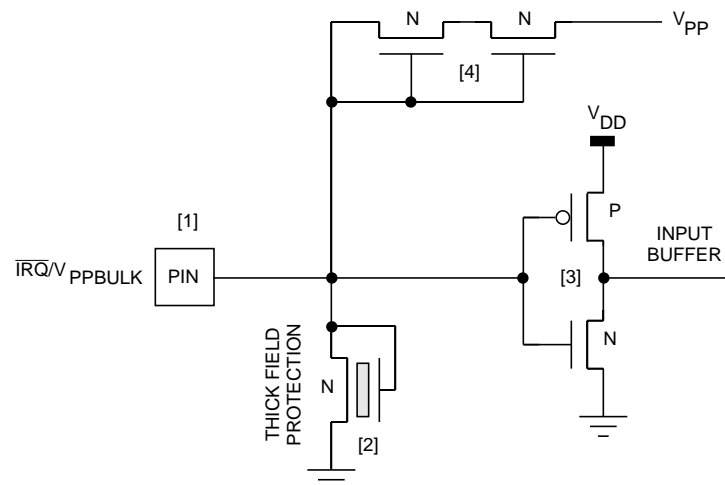
Figure 2-21 Internal Circuitry — \overline{\text{IRQ}}/\text{V}_{\text{PPBULK}} Pin
