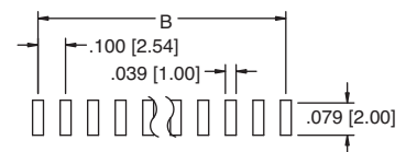
PH1RB-10-UA-SMT
