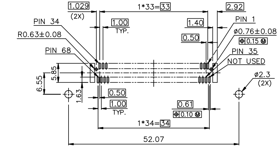
(RECOMMENDED PCB LAYOUT FOR CONAN)
