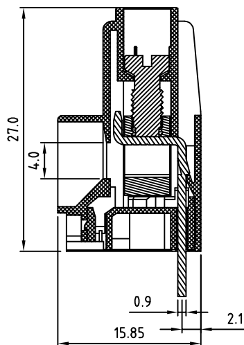
SECTION C-C
