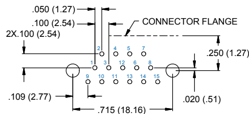
15 PIN
