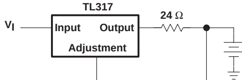
Figure 7. 50-mA Constant-Current Battery Charger Circuit
