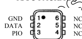
TOP VIEW 3.7 X 4.0 X 1.5
