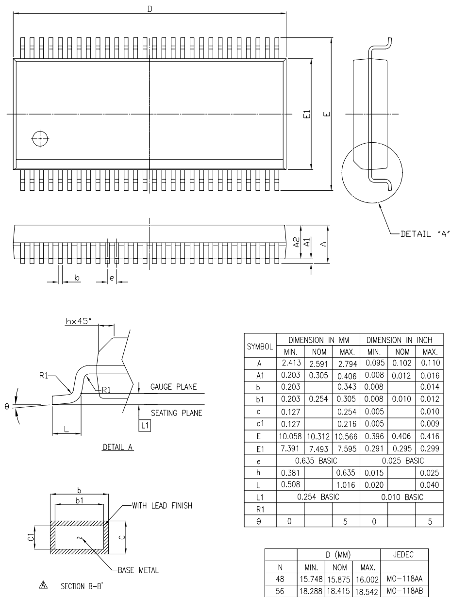
48-Pin SSOP (SM)
