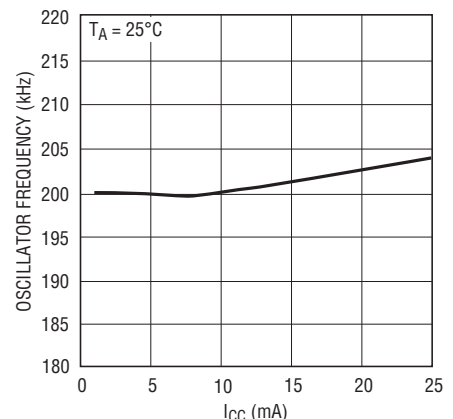
Oscillator Frequency vs V_{CC} Shunt Regulator Current
