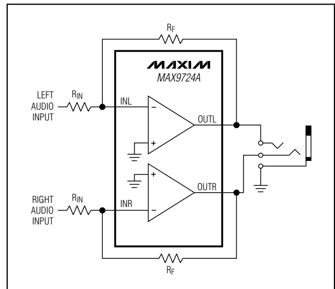
Figure 3. Gain Setting for the MAX9724A
