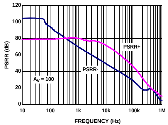
FIGURE 14. ISL28272 PSRR vs FREQUENCY
