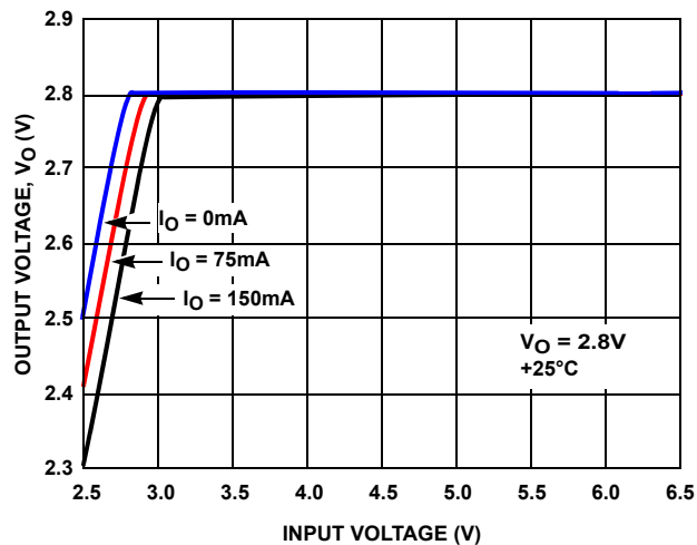
FIGURE 6. DROPOUT VOLTAGE vs INPUT VOLTAGE (2.8V OUTPUT)
