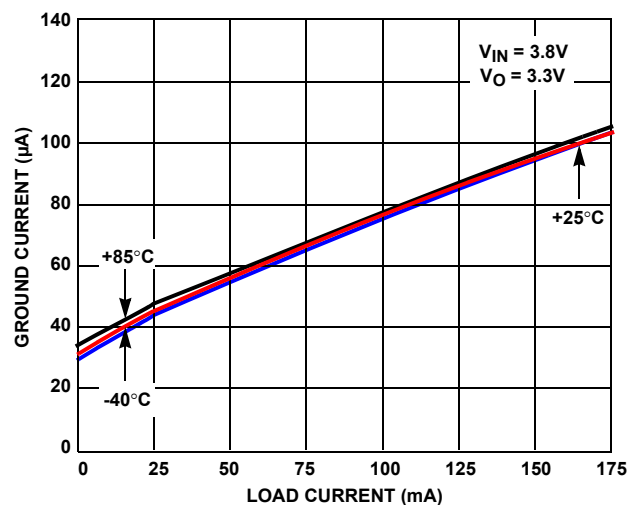
FIGURE 10. GROUND CURRENT vs LOAD
