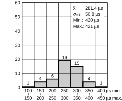
Terminal No. 8-9-10: OFF
