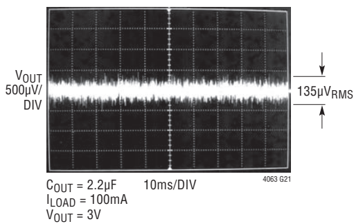
LDO Regulator 10Hz to 100kHz Output Noise
