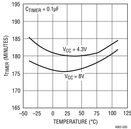
Internal Charge Timer vs Temperature
