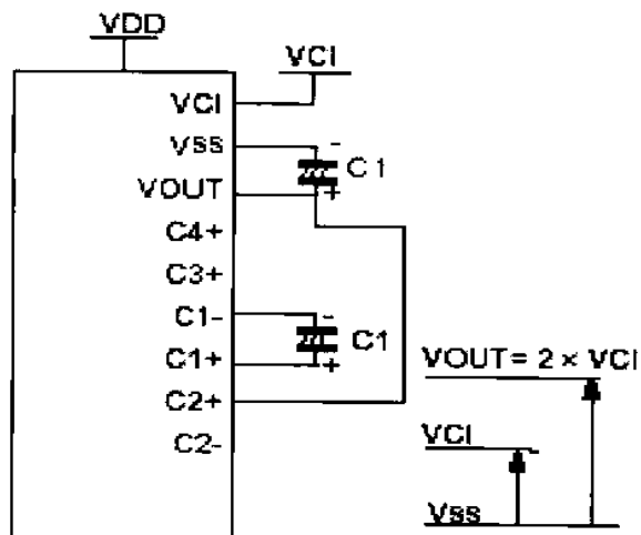
Two Times Boosting Circuit
