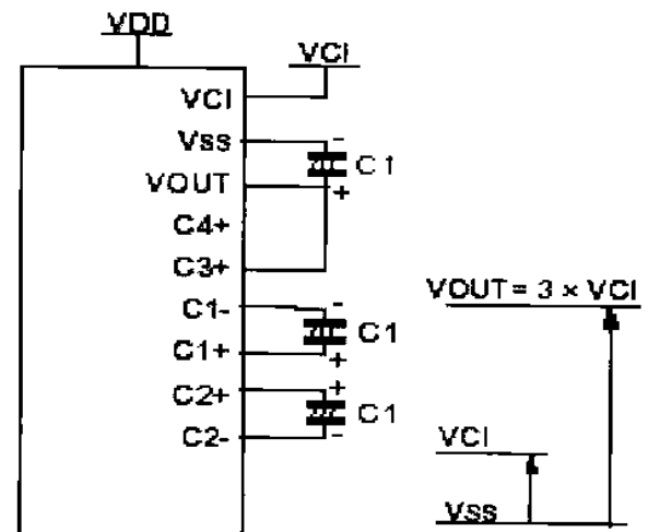
Three Times Boosting Circuit
