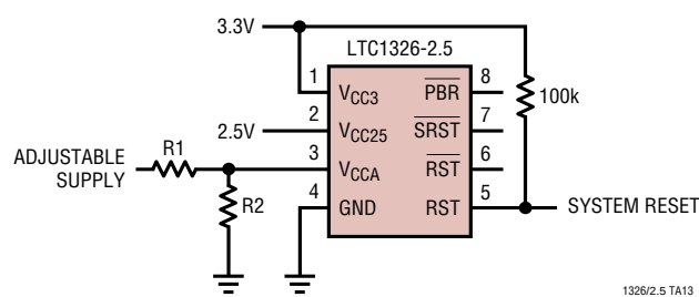
Reset Valid for V_{CC3} Down to 0V
