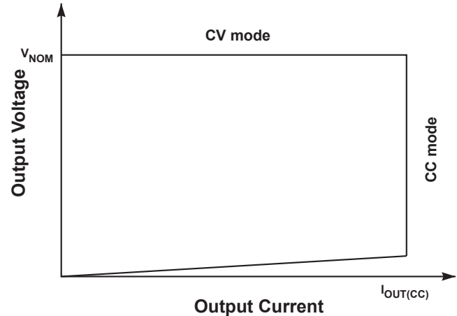
Figure 9.5 : Power Envelope
