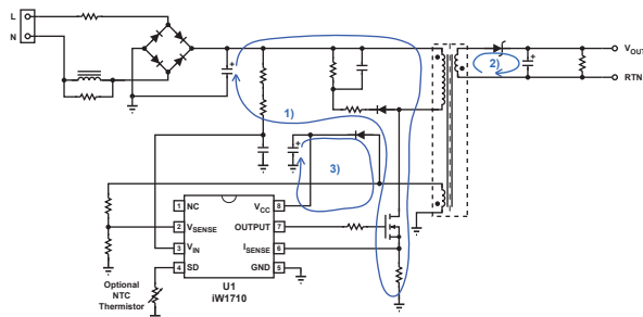
Figure 10.4 : Switching Loops
