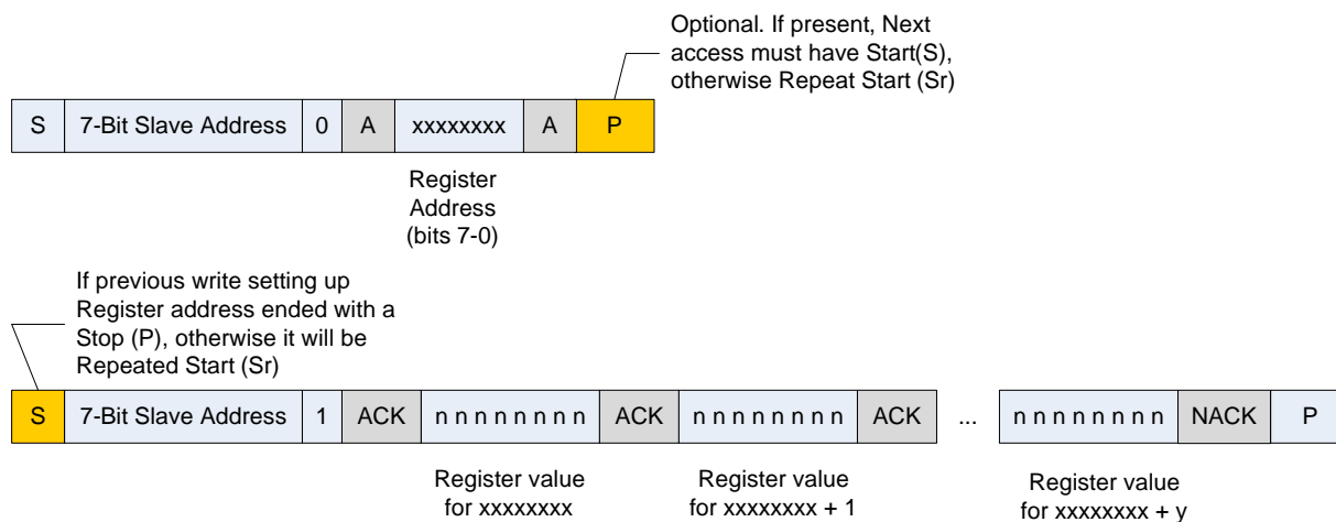
Figure 7.8 I 2 C Sequential Access Read Format
