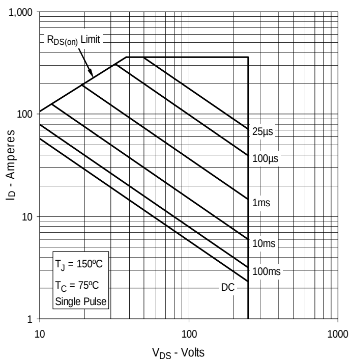
Fig. 14. Forward-Bias Safe Operating Area @ T_C = 75^\circ\text{C}
