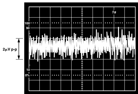
TPC 21. ADR290 0.1 Hz to 10 Hz Noise
