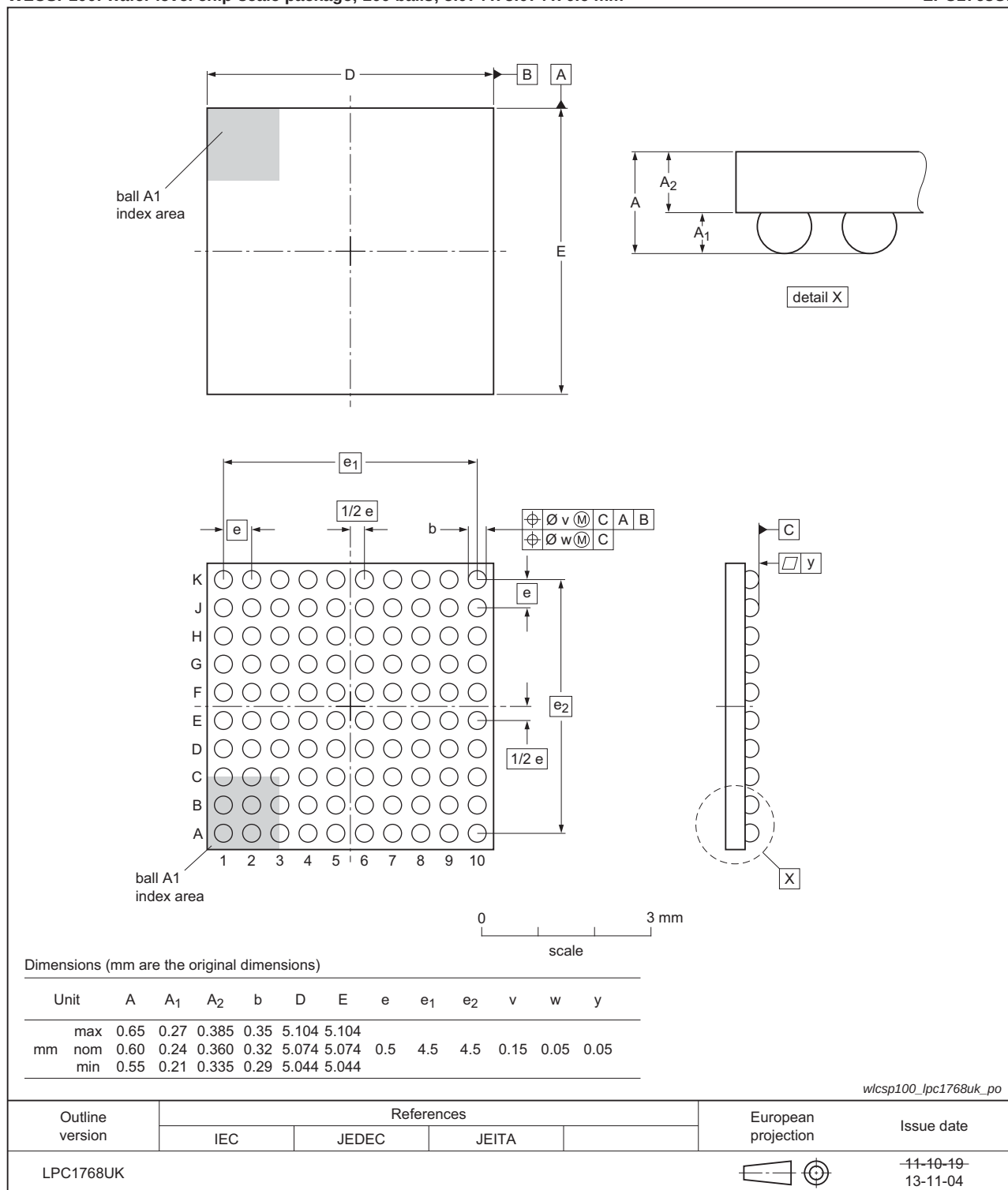
Fig 41. Package outline LPC1768UK (WLCSP100)
