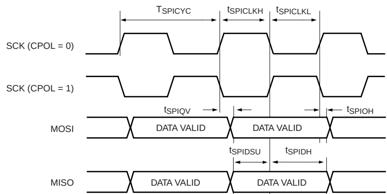
Fig 23. SPI master timing (CPHA = 1)
