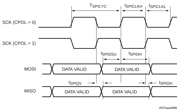
Fig 26. SPI slave timing (CPHA = 0)
