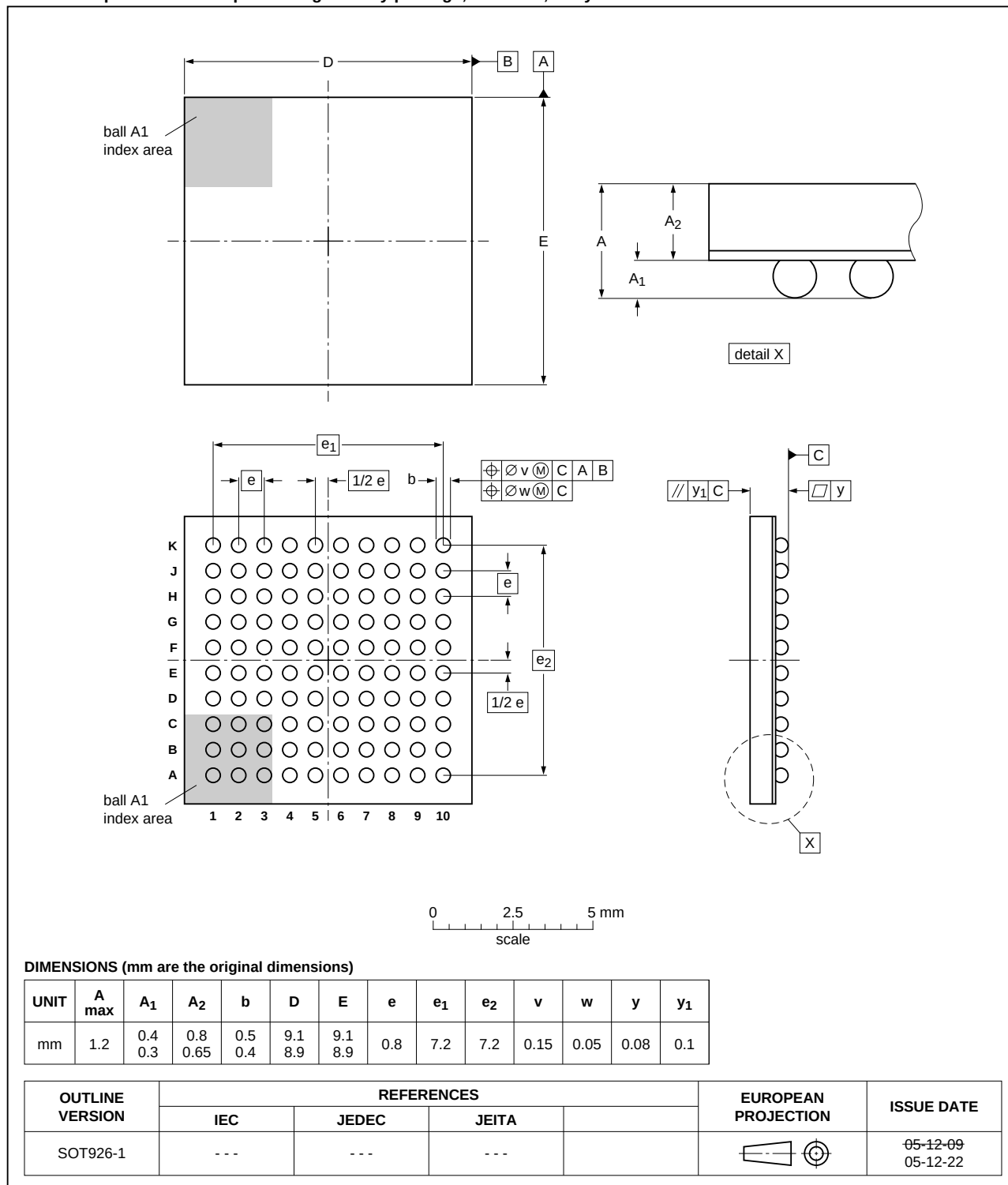
Fig 40. Package outline SOT926-1 (TFBGA100)
