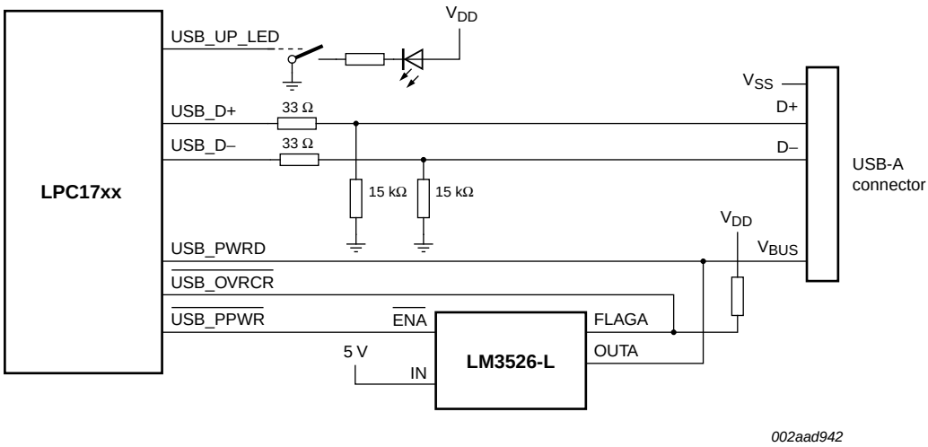
Fig 33. USB host port configuration
