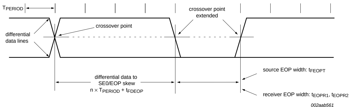
Fig 22. Differential data-to-EOP transition skew and EOP width
