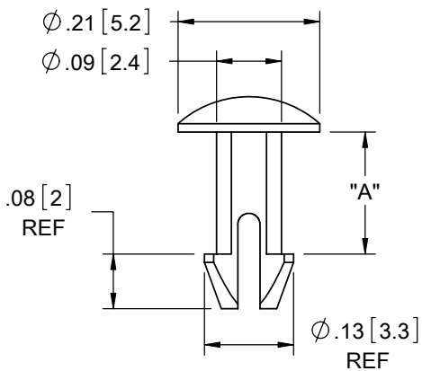
FIG 2. SLP-1-100 SERIES
