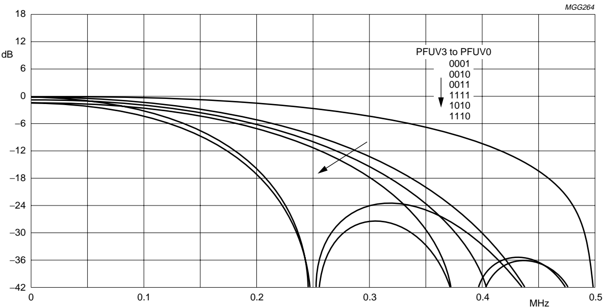
Fig.20 Chrominance Prefilter: frequency response for miscellaneous register settings.
