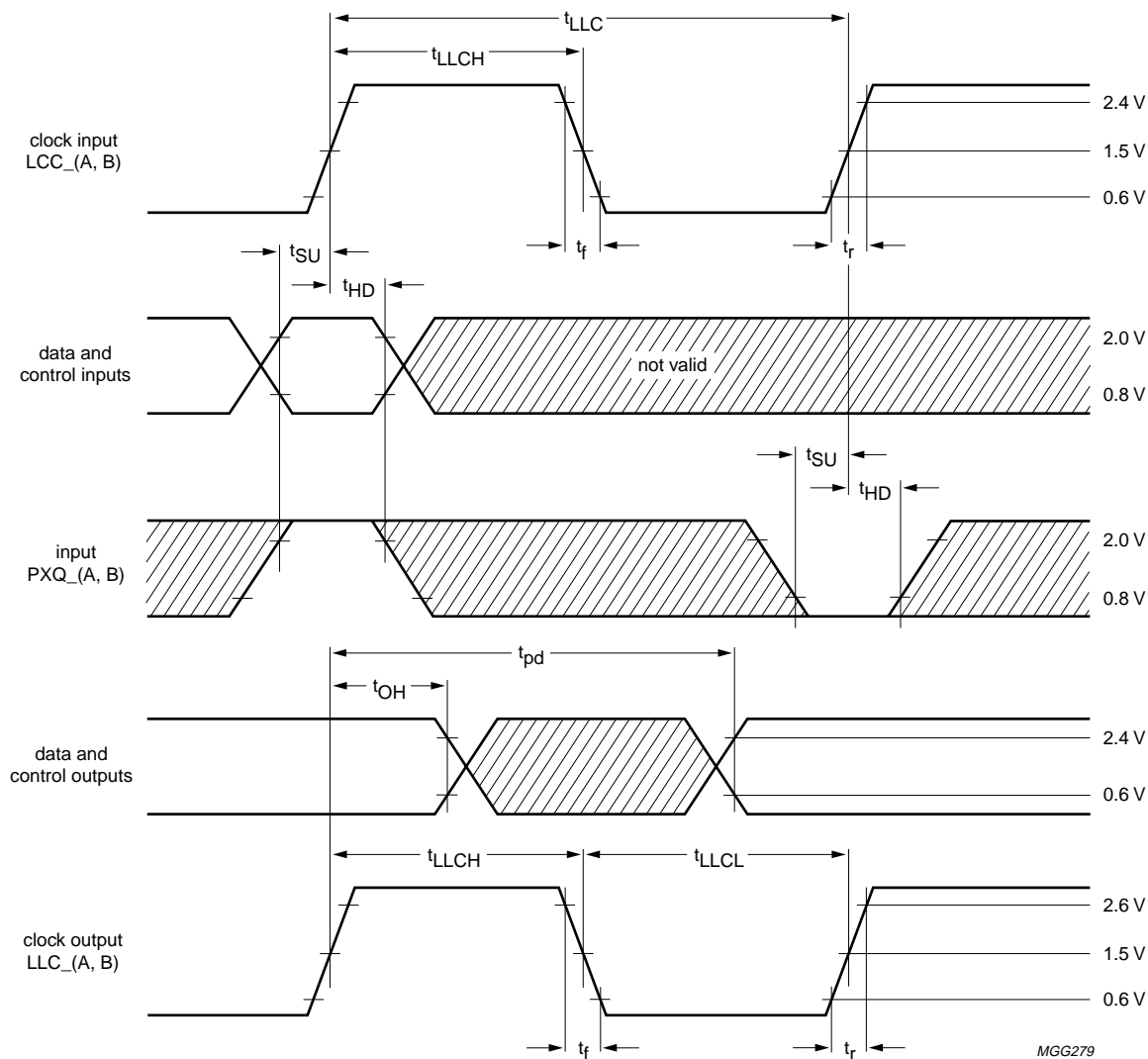
Fig.47 Clock/data timing.
