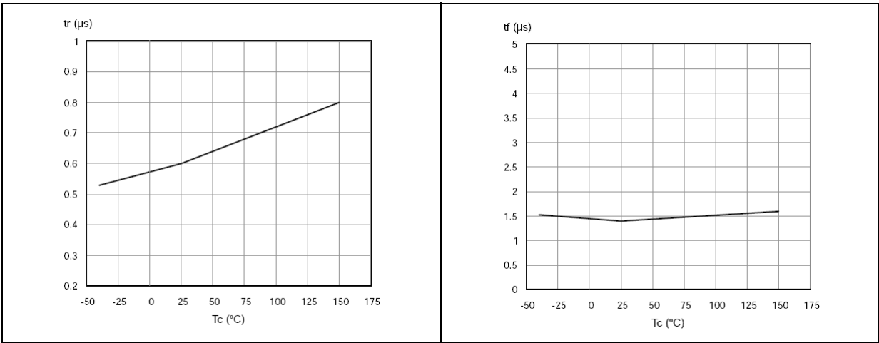
Figure 29. Output voltage rise time Figure 30. Output voltage fall time
