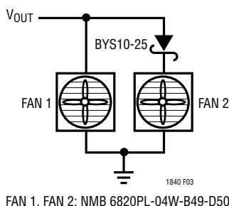
Figure 3. Series Diode to Avoid Beat Frequencies
