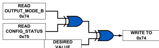
FIGURE 41. SETTING OUTPUT_MODE_B REGISTER
