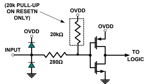
FIGURE 45. DIGITAL INPUTS
