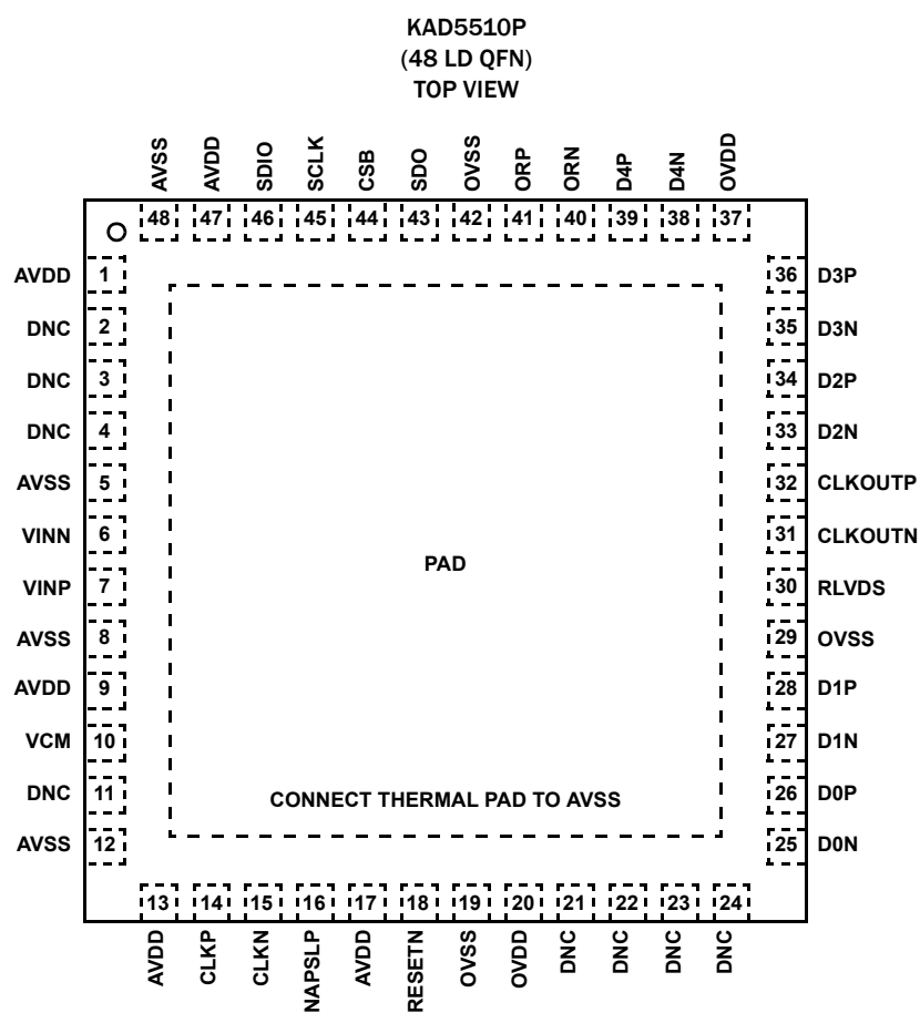
FIGURE 1. PIN CONFIGURATION
