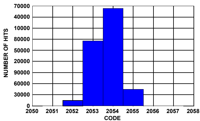
FIGURE 14. NOISE HISTOGRAM
