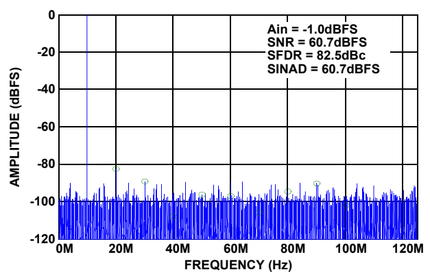
FIGURE 15. SINGLE-TONE SPECTRUM @ 10MHz
