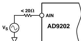
Figure 26. Simple Drive Configuration
