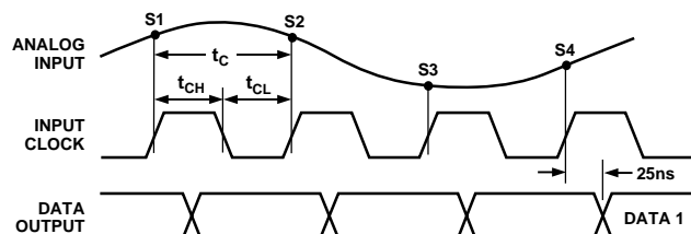
Figure 30. Timing Diagram
