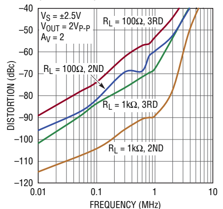
Distortion vs Frequency ( A_V = 2, 5V )
