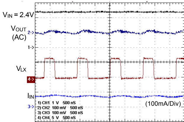
Stability for Driving 1 WLED
