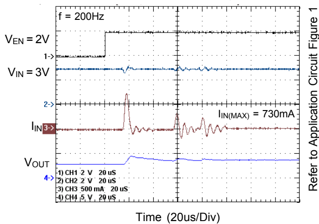
Inrush Current for Driving 1 WLED
