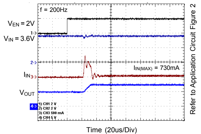
Inrush Current for Driving 2 WLEDs
