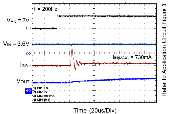
Inrush Current for Driving 3 WLEDs with soft-start
