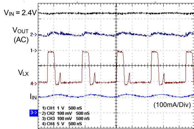
Stability for Driving 3 WLEDs
