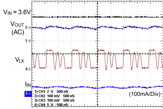
Stability for Driving 2 WLEDs
