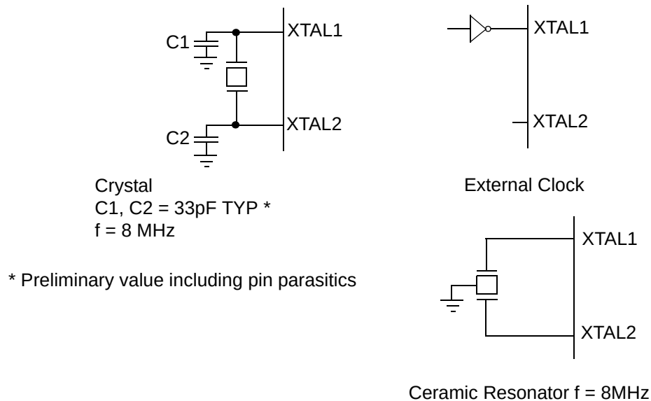
Figure 31. Oscillator Configuration
