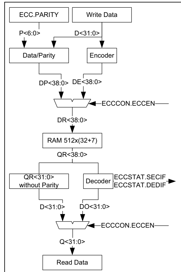
FIGURE 3-3: ECC LOGIC
