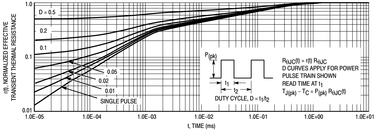
Figure 13. Thermal Response
