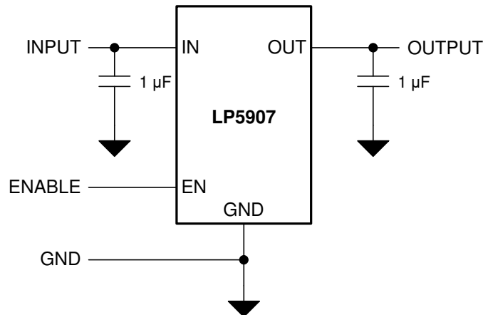
Simplified Schematic
