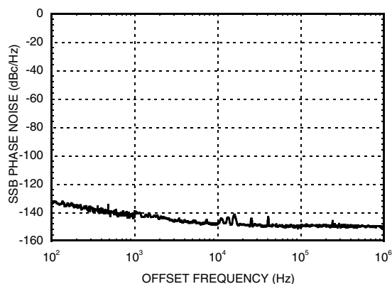
SSB Phase Noise Performance, P_{in} = 0\text{ dBm} , F_{in} = 22\text{ GHz} , T = 25^\circ\text{C}
