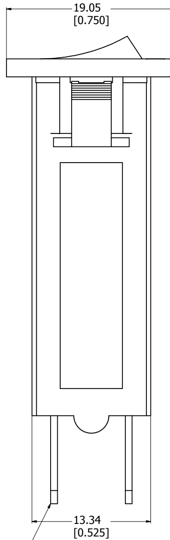
SIDE VIEW
