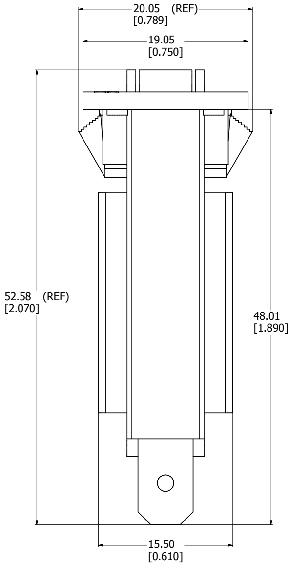
FRONT VIEW
