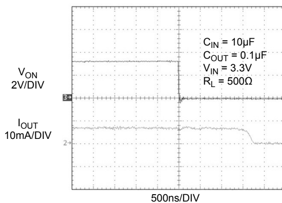
Figure 16. T_{OFF} Response
