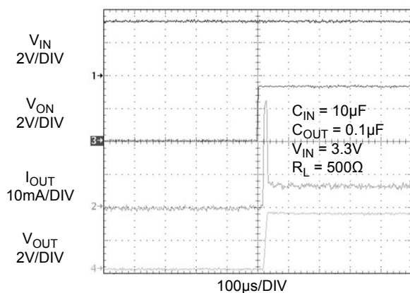
Figure 15. T_{ON} Response
