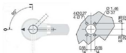
Front operation Direction of operation Door drilling template
