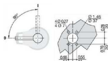
Side operation Direction of operation Door drilling template
