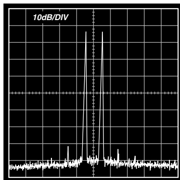
Figure 23. Third Order Intermodulation Distortion at 10.7 MHz (10 \times Probe Used to HP3585A Spectrum Analyzer, Gain = 0 dB, P_{IN} = 0 dBm, Pin 5 Connected to Pin 7)
