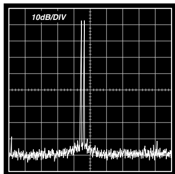
Figure 22. Third Order Intermodulation Distortion at 455 kHz (10 \times Probe Used to HP3585A Spectrum Analyzer, Gain = 0 dB, P_{IN} = 0 dBm, Pin 5 Connected to Pin 7)
