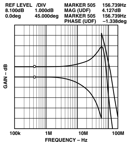
Figure 17. Frequency and Phase Response vs. Gain (Gain = -10 dB, P_{IN} = -30 dBm, Pin 5 Connected to Pin 7)
