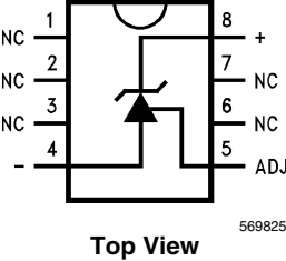
8-Pin SOIC Surface Mount Package
