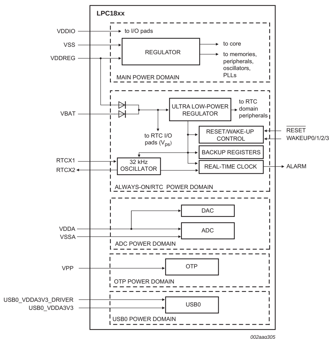
Fig 10. LPC1850/30/20/10 power domains
