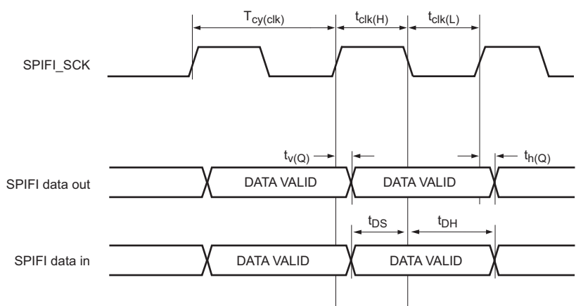
Fig 39. SPIFI timing
