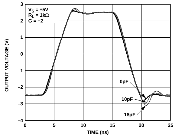
Figure 40. Large Signal Transient Response with Capacitive Load
