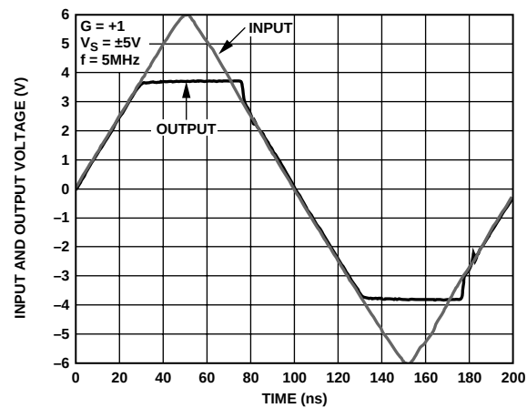
Figure 42. Input Overdrive Recovery
