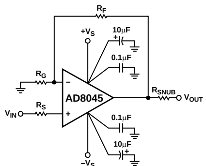
Figure 61. Noninverting Configuration
