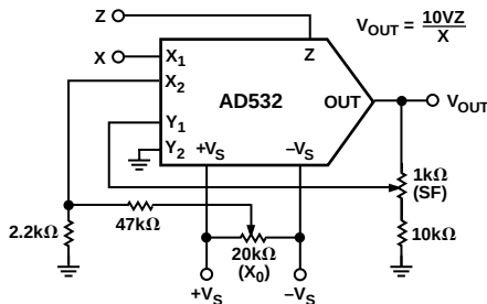
Figure 13. Divider Connection
