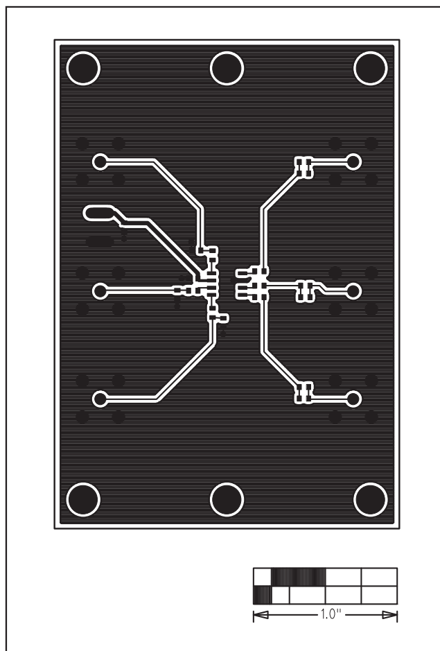
Figure 3. MAX9652 EV Kit PCB Layout—Component Side
