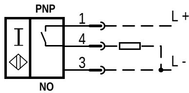
3RG40133AG01 / 3RG40132AG01:
