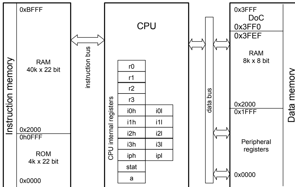
Figure 4 - Memory organization
