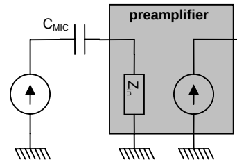
Figure 32 - Equivalent schematic for C_{MIC} calculation
