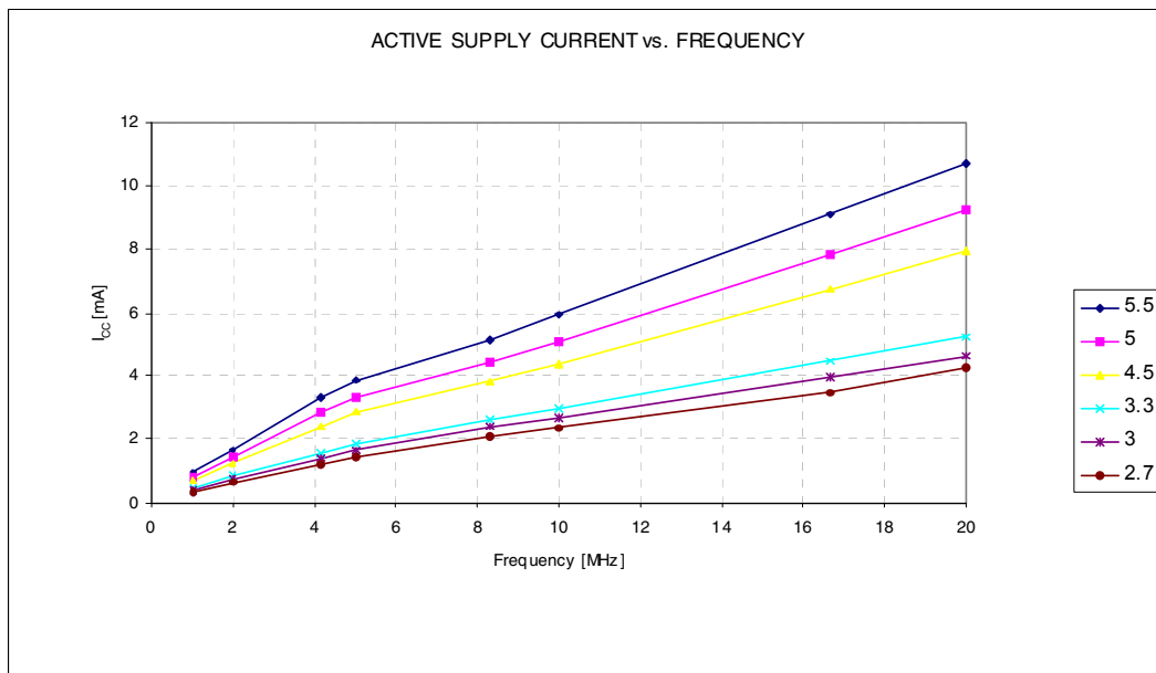
Figure 22-1. Active Supply Current vs.Frequency (0 - 16 MHz)
