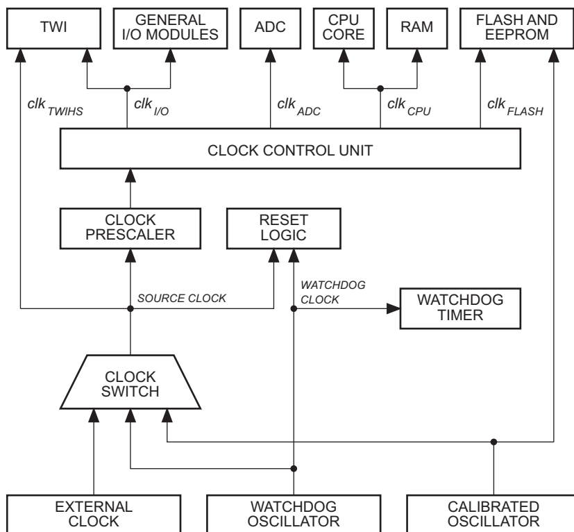
Figure 6-1. Clock Distribution
