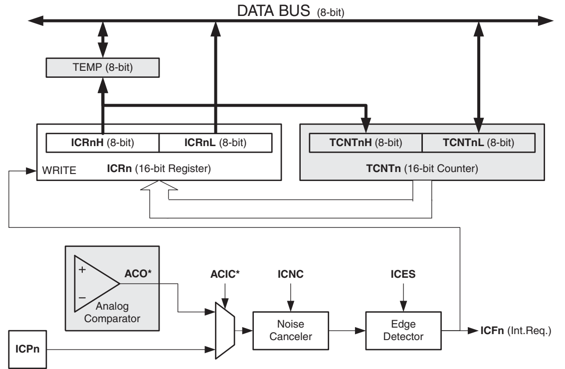
Figure 12-3. Input Capture Unit Block Diagram
