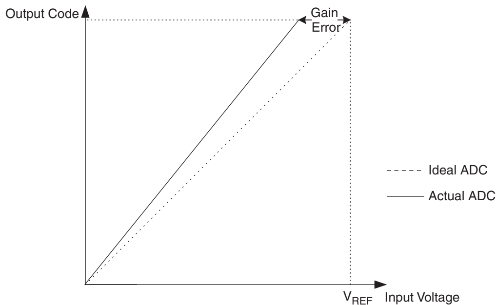
Figure 17-11. Gain Error
