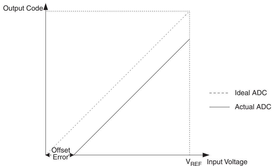
Figure 17-10. Offset Error
