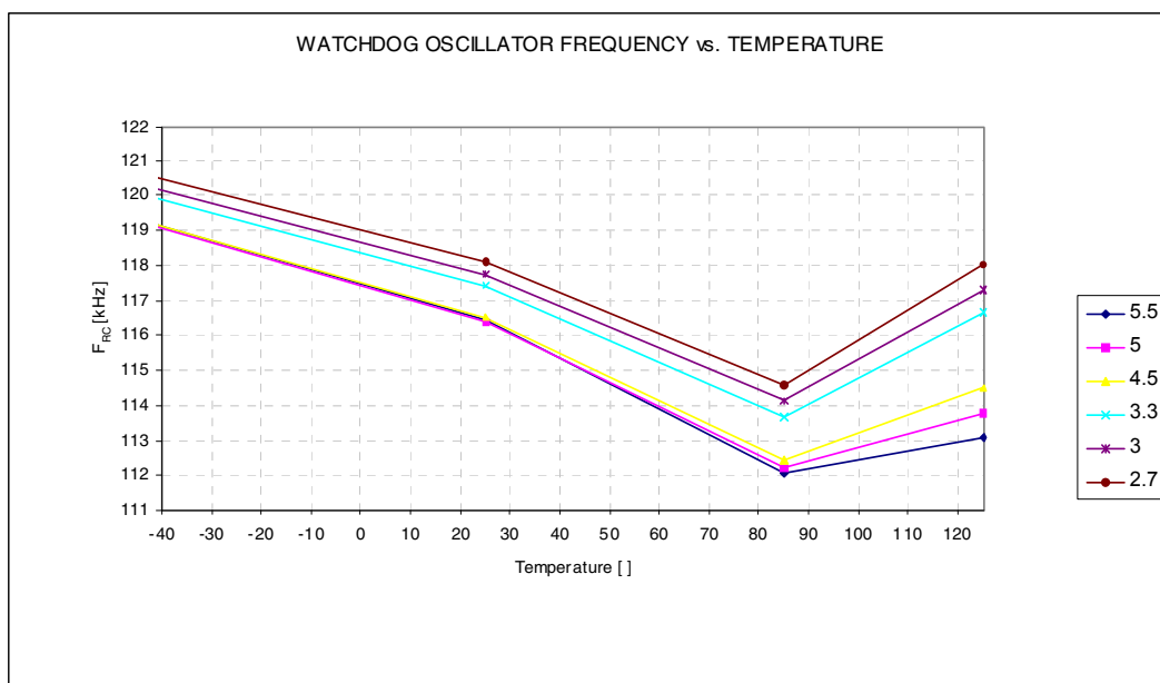
Figure 22-17. Watchdog Oscillator Frequency vs. Temperature
