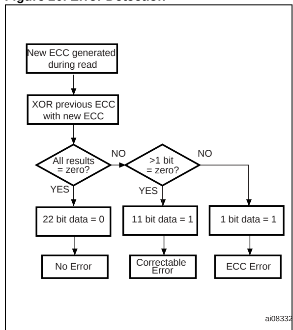
Figure 20. Error Detection
