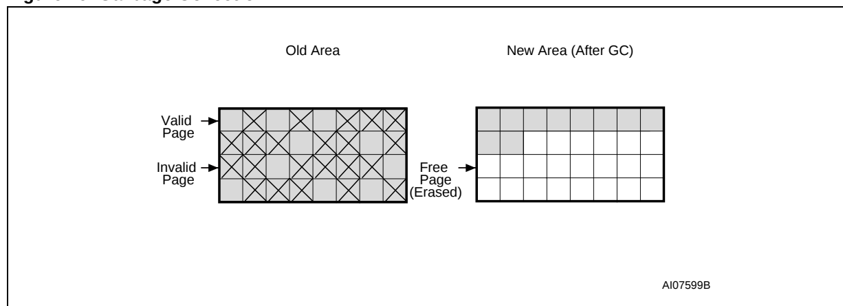
Figure 19. Garbage Collection
