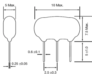
Figure 1) ZTT□.□□MG Side and Front Views
