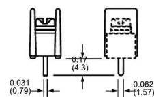
08 Printed Circuit
